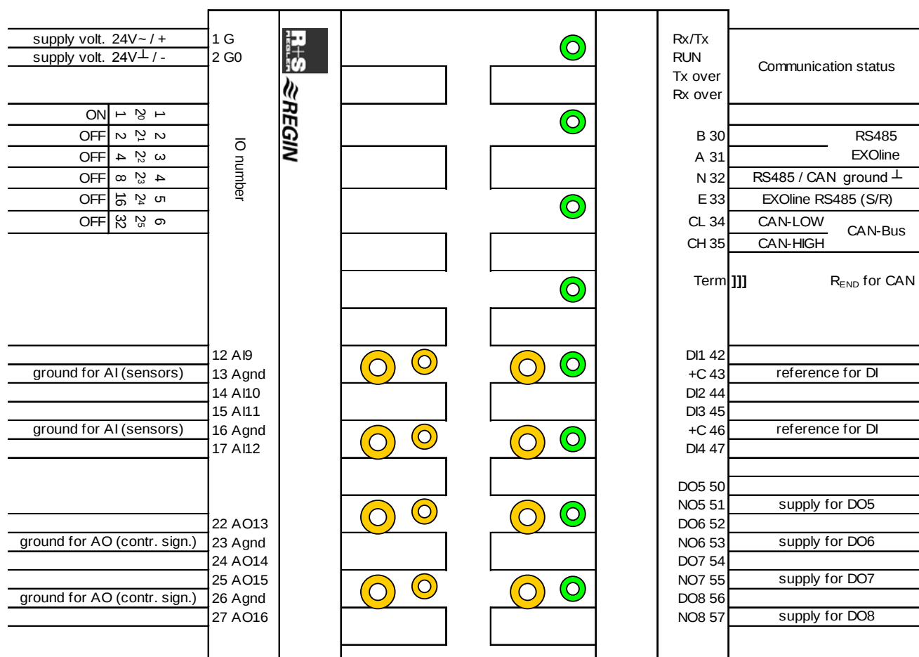
Fig. 6: IO-4X4-M terminals
