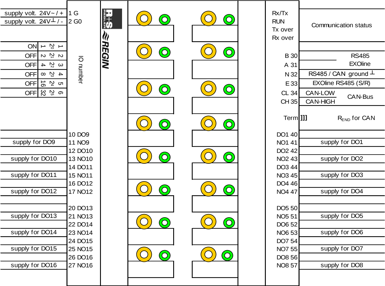
Fig. 3: IO-16DO-M terminals
