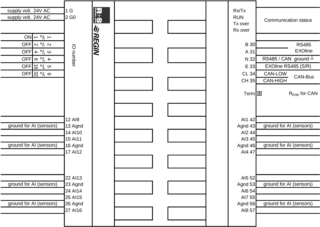
Fig. 1: IO-16AI terminals
