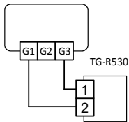
Fig. 3 Room sensor and internal setpoint
