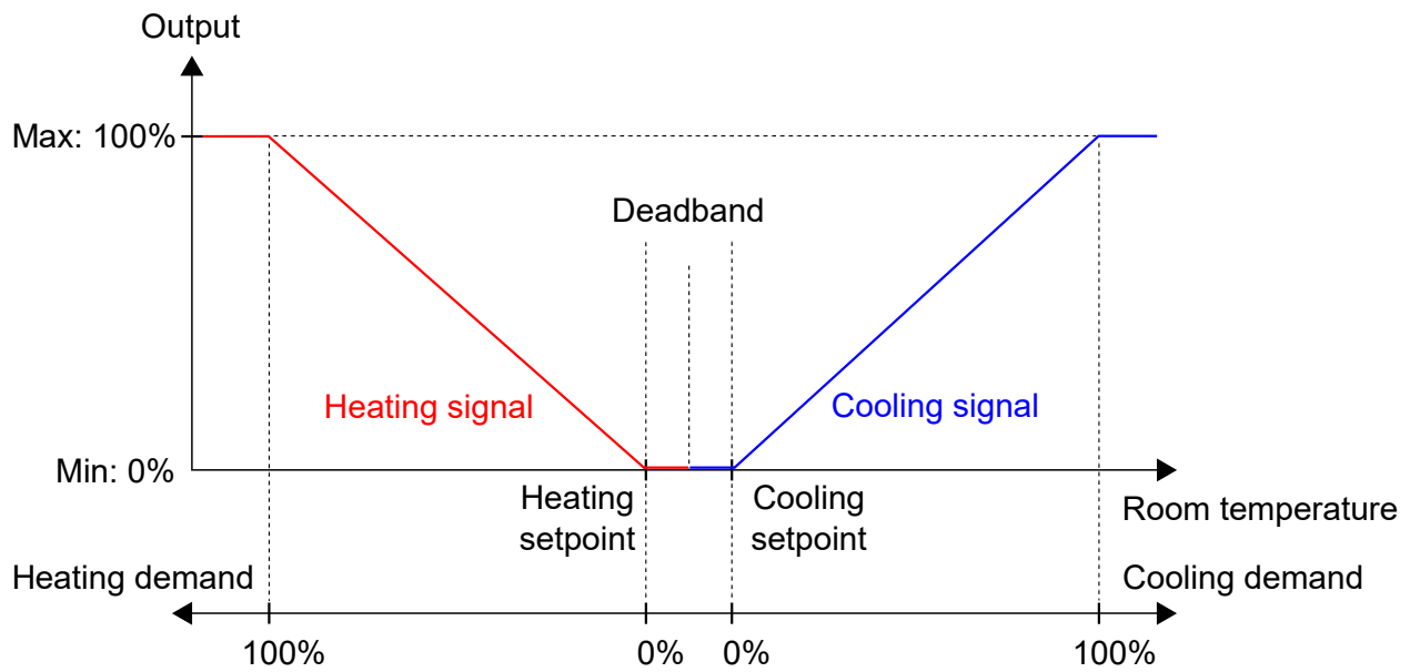
Figure 3-39 Control behaviour for the Heating + Cooling controller mode
