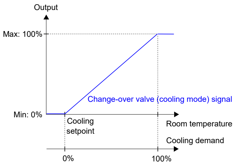
Figure 3-44 Control behaviour for the Heating/Cooling (change-over) controller sequence when the controller is in cooling mode
