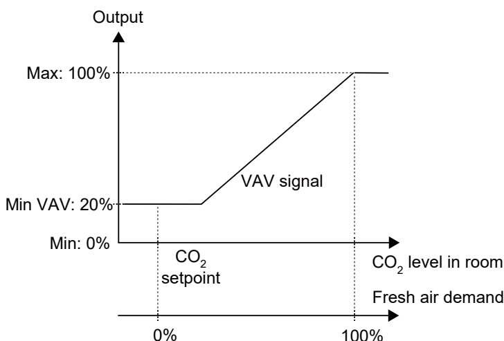
Figure 3-47 CO 2 control behaviour
