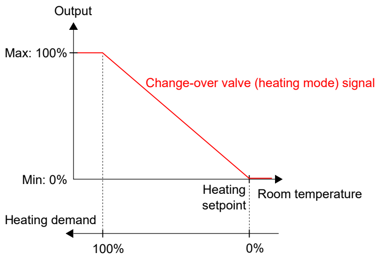
Figure 3-43 Control behaviour for the Heating/Cooling (change-over) controller sequence when the controller is in heating mode
