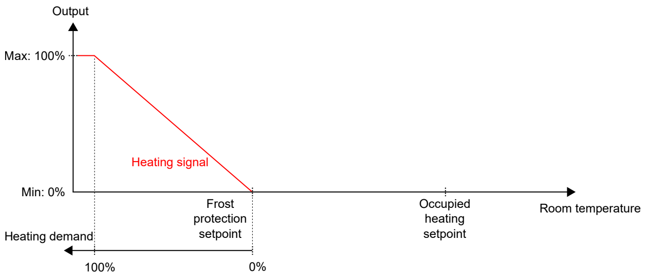
Figure 3-13 Control behaviour for the off controller state
