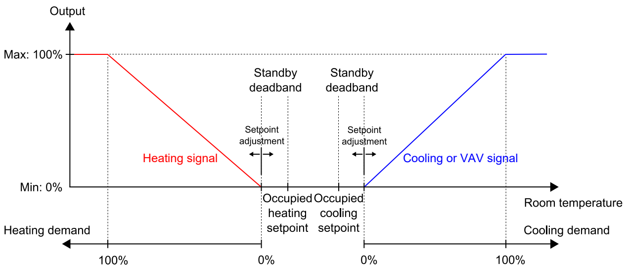
Figure 3-15 Control behaviour for the standby controller state
