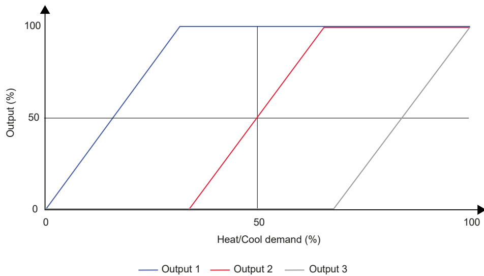
Figure 3-19 Three Heat/Cool sequences behaviour
