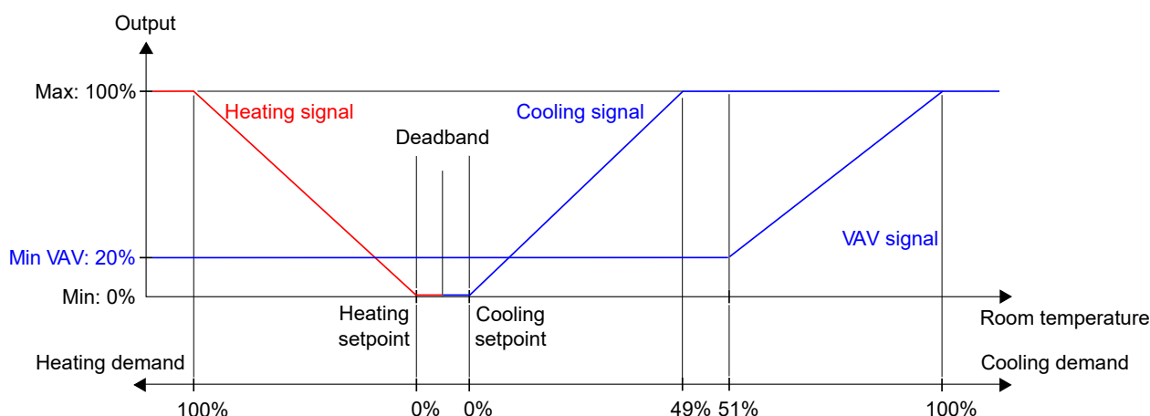
Figure 3-46 Control behaviour for the Heating + Cooling + VAV controller mode when the controller regulates based on heating and cooling demand
