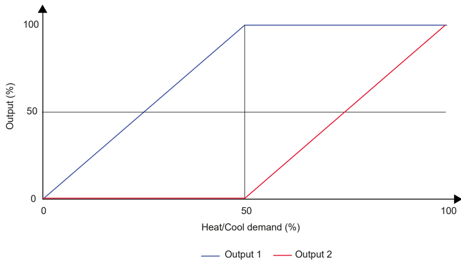
Figure 3-18 Two Heat/Cool sequences behaviour
