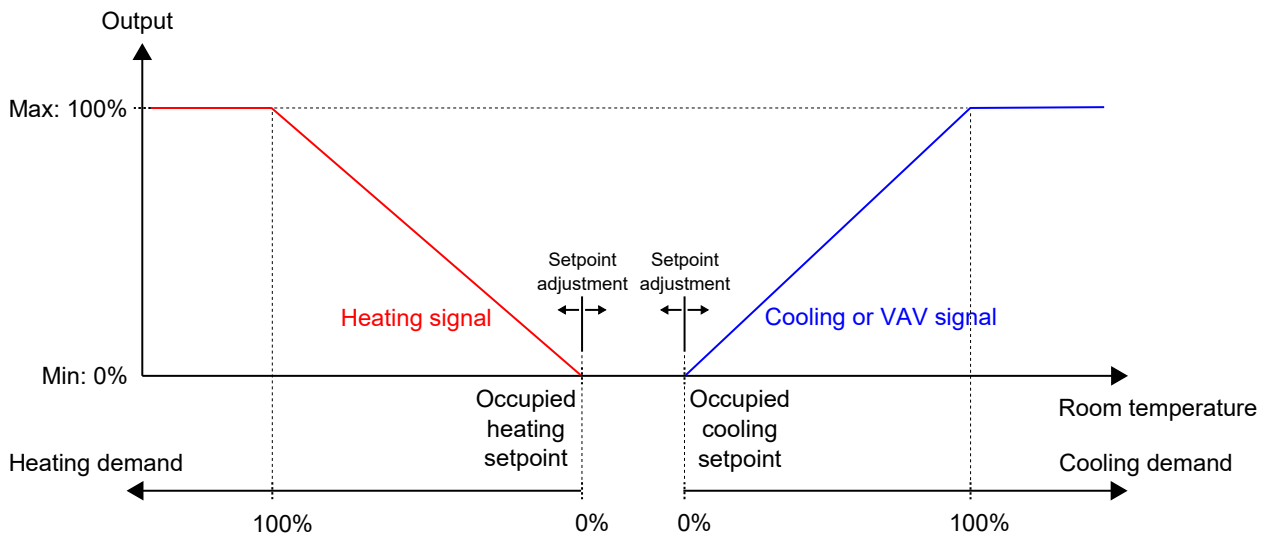
Figure 3-16 Control behaviour for the occupied and Forced ventilation controller state
