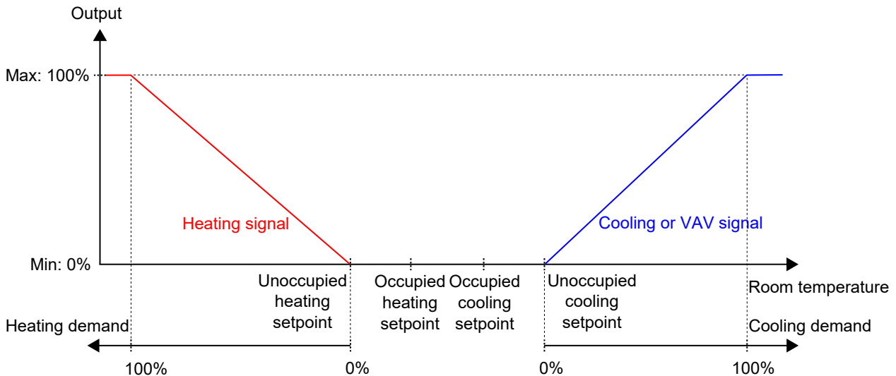
Figure 3-14 Control behaviour for the unoccupied controller state
