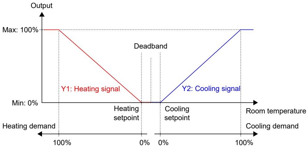
Figure 3-41 Control behaviour for the Heating + Cooling controller sequence
