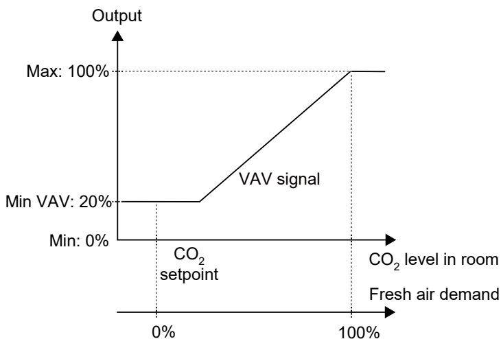
Figure 3-36 CO 2 control behaviour
