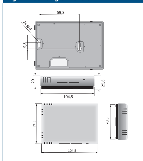
Fig. 2 Mounting dimension
