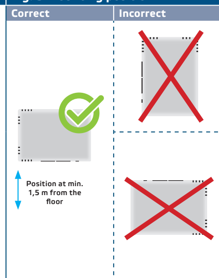
Fig. 3 Mounting position
