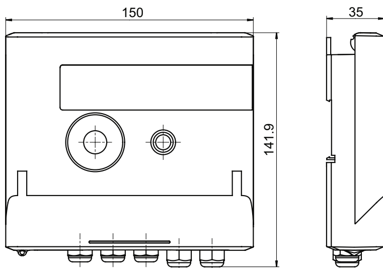
Fig. 7 Calculator
