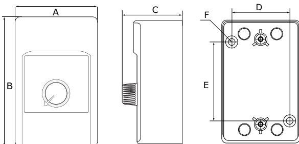
Fig. 1 Mounting dimensions
